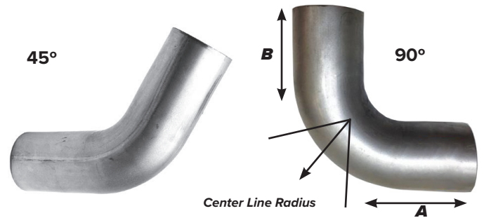
45° ELBOWS (O.D.-O.D.)
