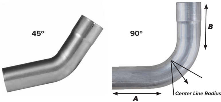
45° ELBOWS (I.D.-O.D.)
